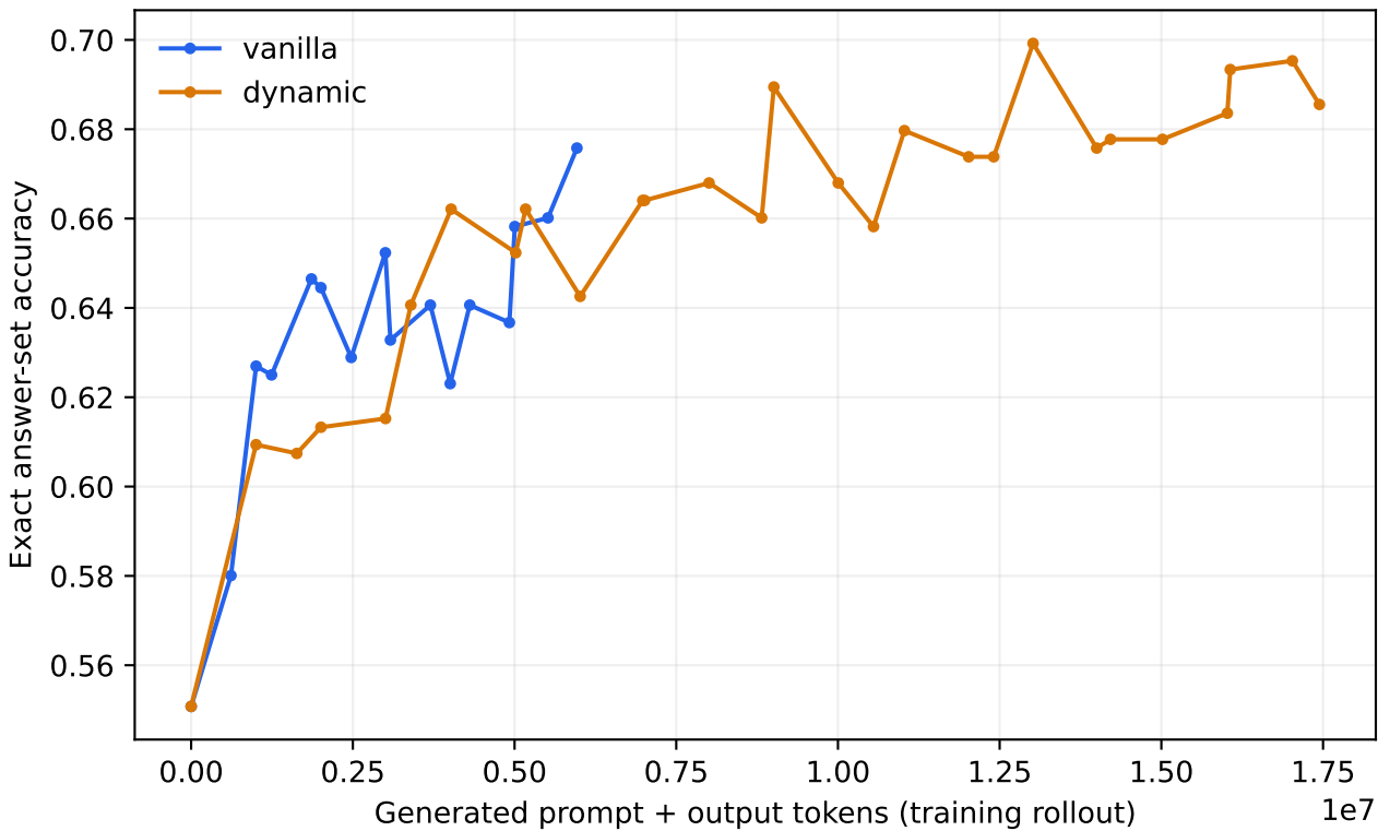
FORMAL · validation accuracy vs generated total tokens
