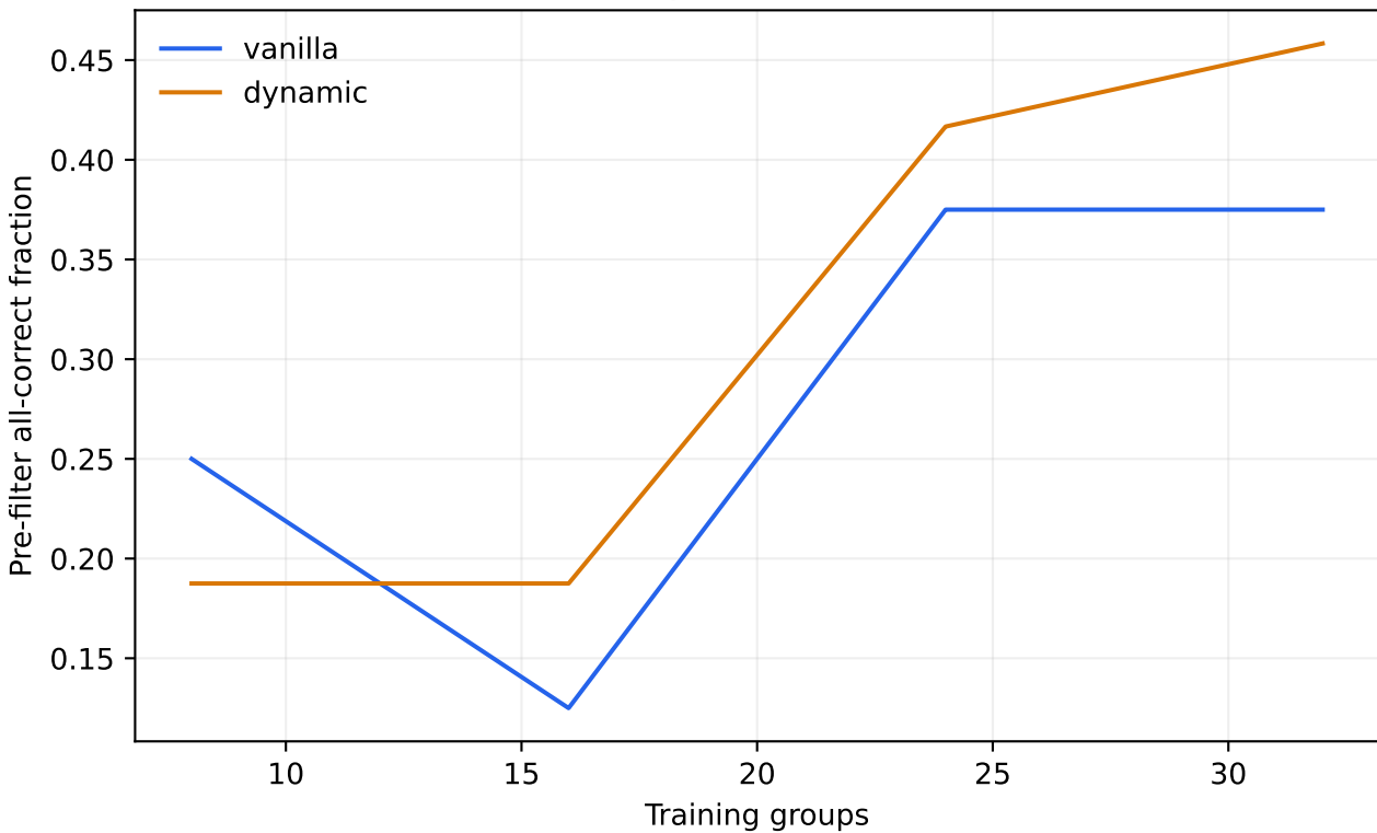
SMOKE · pre filter all correct
