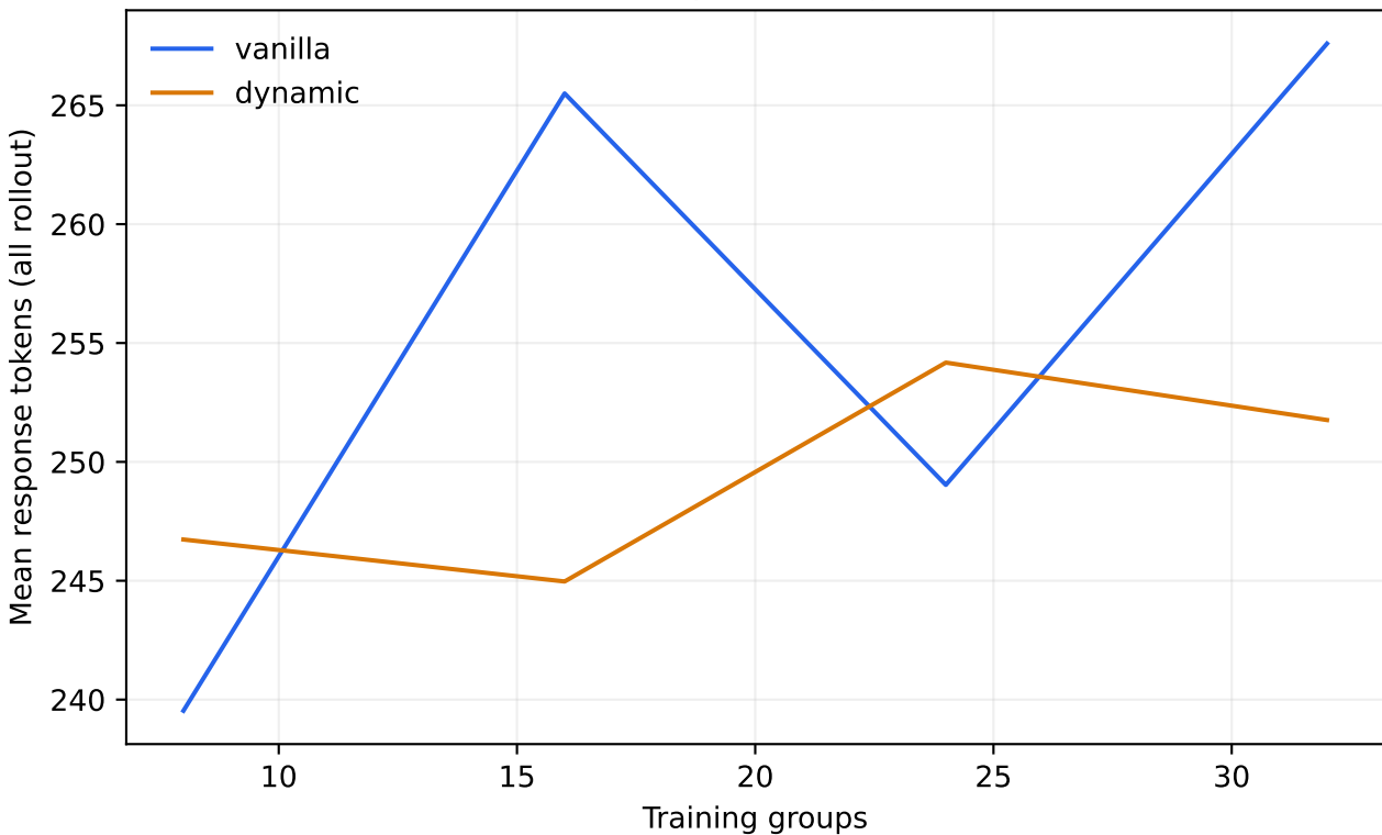
SMOKE · response length mean
