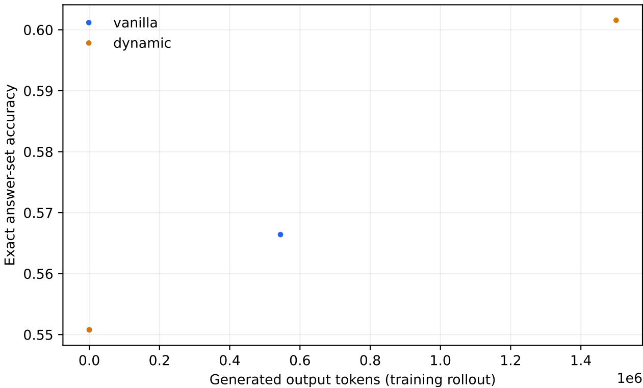
PILOT · validation accuracy vs generated output tokens
