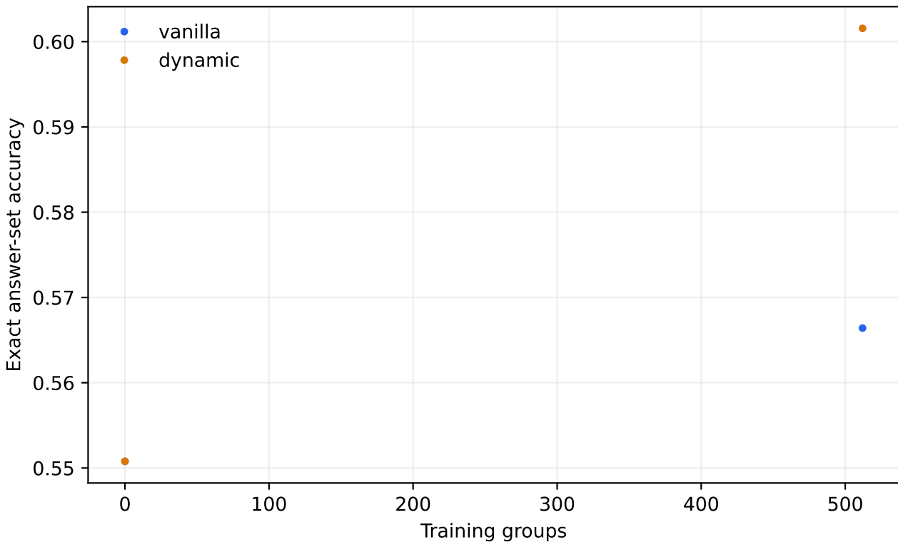
PILOT · validation accuracy vs training groups
