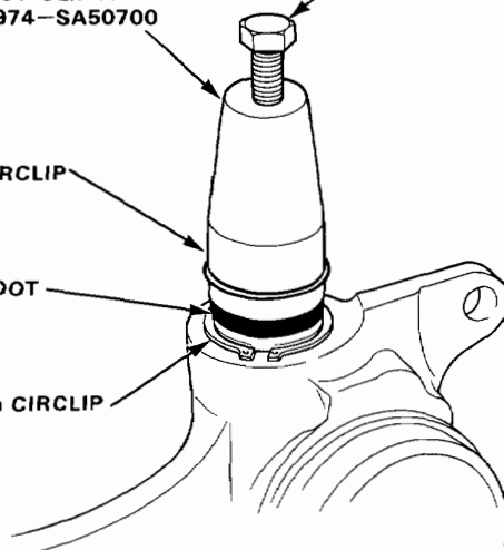
BALL JOINT BOOT CLIP A 07974-SA50700
