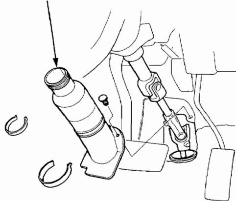
STEERING JOINT COVER
