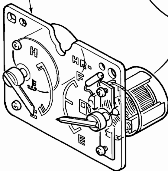
FUEL GAUGE/COOLANT TEMPERATURE GAUGE
