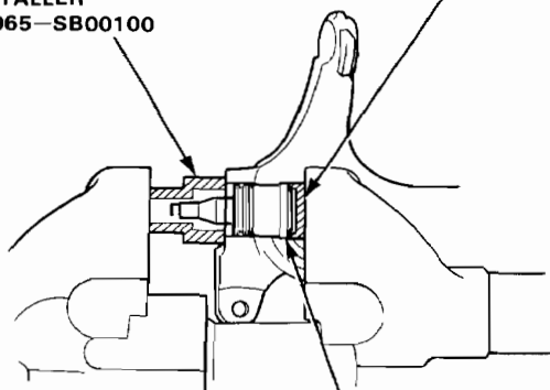
BALL JOINT REMOVER/ INSTALLER 07965-SB00100
