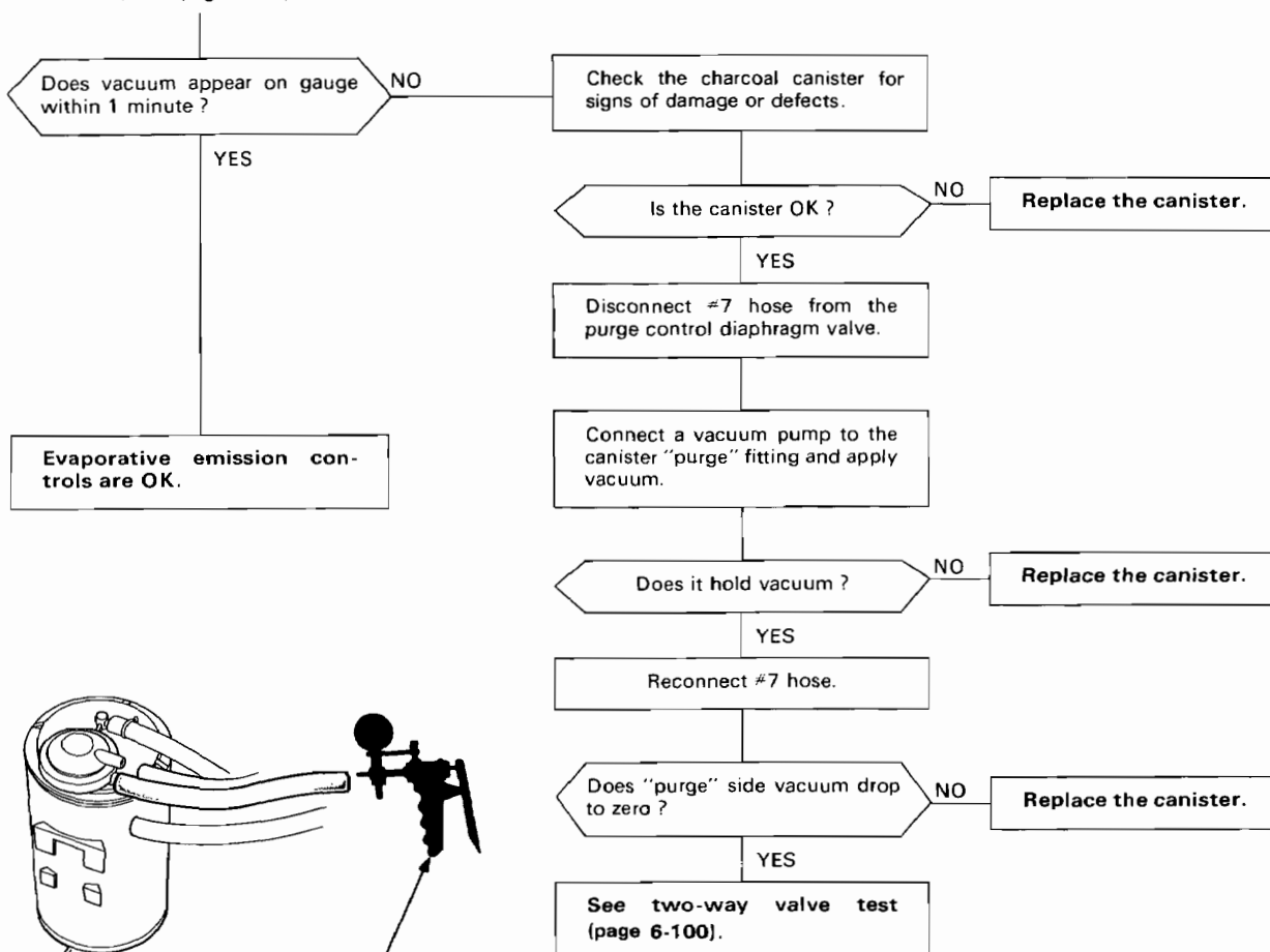
VACUUM PUMP/GAUGE
