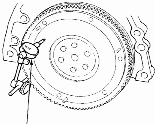
DIAL INDICATOR
