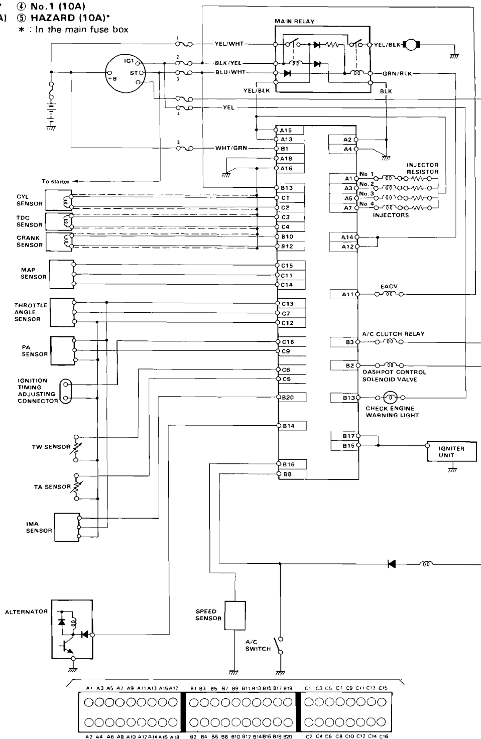
TERMINAL LOCATION
