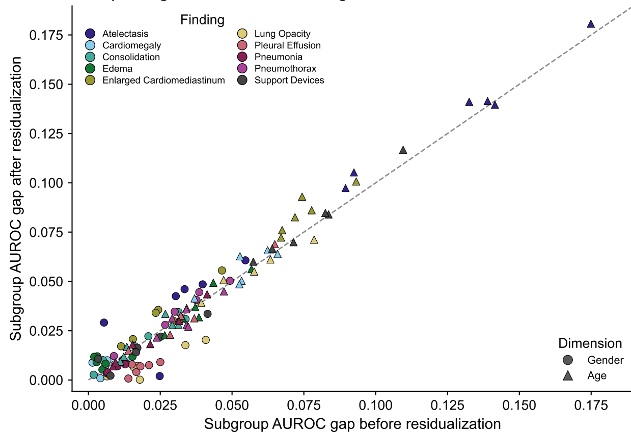
A. Gap change at each model × finding × dimension cell
