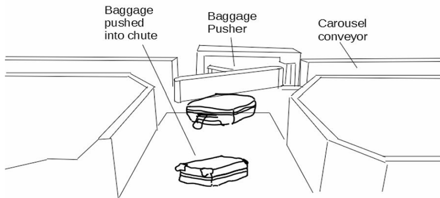
Figure 2: Carousel sorter
