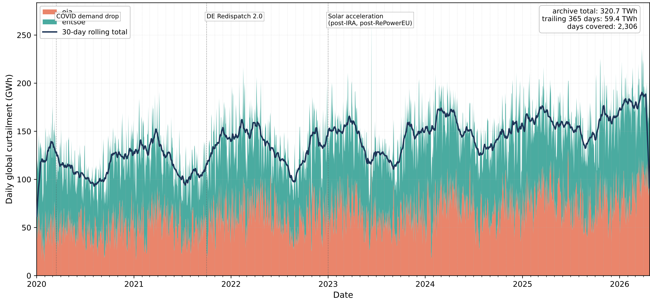
Figure 3. Daily global curtailment from HB backfill archive (2020-01-01 to 2026-04-24, n=2306 days, 2 source streams)
