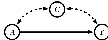
Latent Projection (ADMG)
