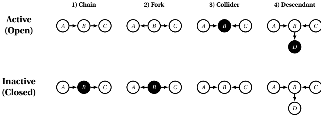
Figure 3.3: The four atomic structures governing the flow of statistical dependence. Paths are active (top row) when chains/forks are unconditioned and colliders/descendants are conditioned. They become inactive (bottom row) when the conditioning is reversed.
