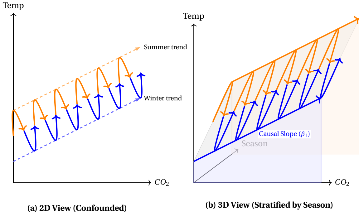
Figure 2.13: Linear regression as covariate adjustment. In 2D space (a), the cyclic confounding of season obscures the true causal step from CO_2 to Temperature. By adding Season as a covariate in a multiple regression (b), we lift the data into 3D space. The regression coefficient ( \beta_1 ) is geometrically equivalent to the slope of a 1D line projected onto a 2D slice where Season is held completely constant.
