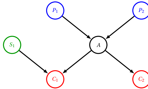
Figure 3.7: The Markov Boundary of node A (black). It consists of its parents \mathbf{PA}(A) , its children \mathbf{CH}(A) , and its co-parents \mathbf{PA}(\mathbf{CH}(A)) . Conditioning on this specific set completely d-separates A from every other node in the graph.
