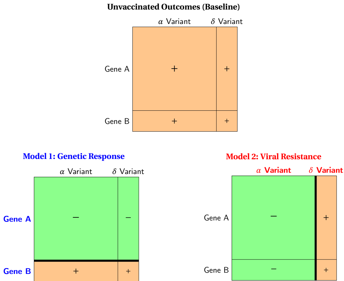
Figure 2.7: Comparison of individual responses to vaccination. The area of each box represents the population proportion. In Model 1 , the outcome is determined entirely by the rows (indicated by the thick blue horizontal divider). In Model 2 , the outcome is determined entirely by the columns (thick red vertical divider). Both yield 90% aggregate effectiveness (90% of the total area is green), but individual counterfactuals diverge drastically.
