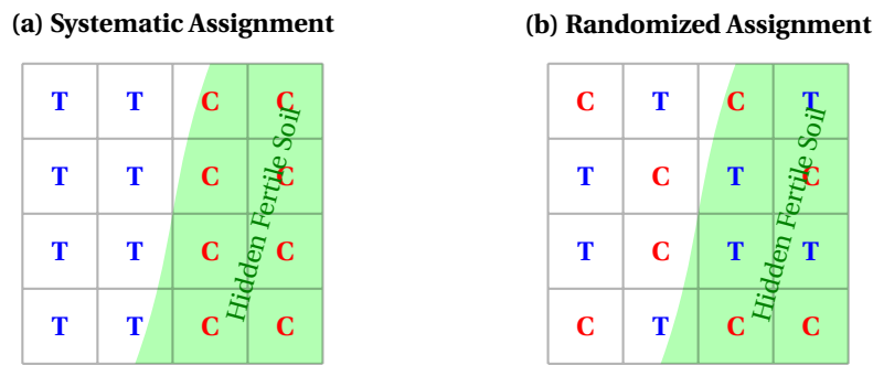
Figure 2.11: Fisher's insight on unobserved confounding in agricultural trials. (a) Systematic assignment perfectly confounds the Control ( C ) group with the hidden fertile soil. (b) Random assignment ensures that both treated and control plots land in the fertile band at approximately equal rates.
