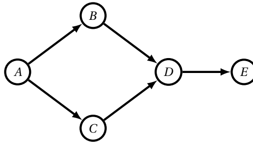
Figure 3.1: A DAG demonstrating multiple valid topological orderings, including (A, B, C, D, E) and (A, C, B, D, E) .
