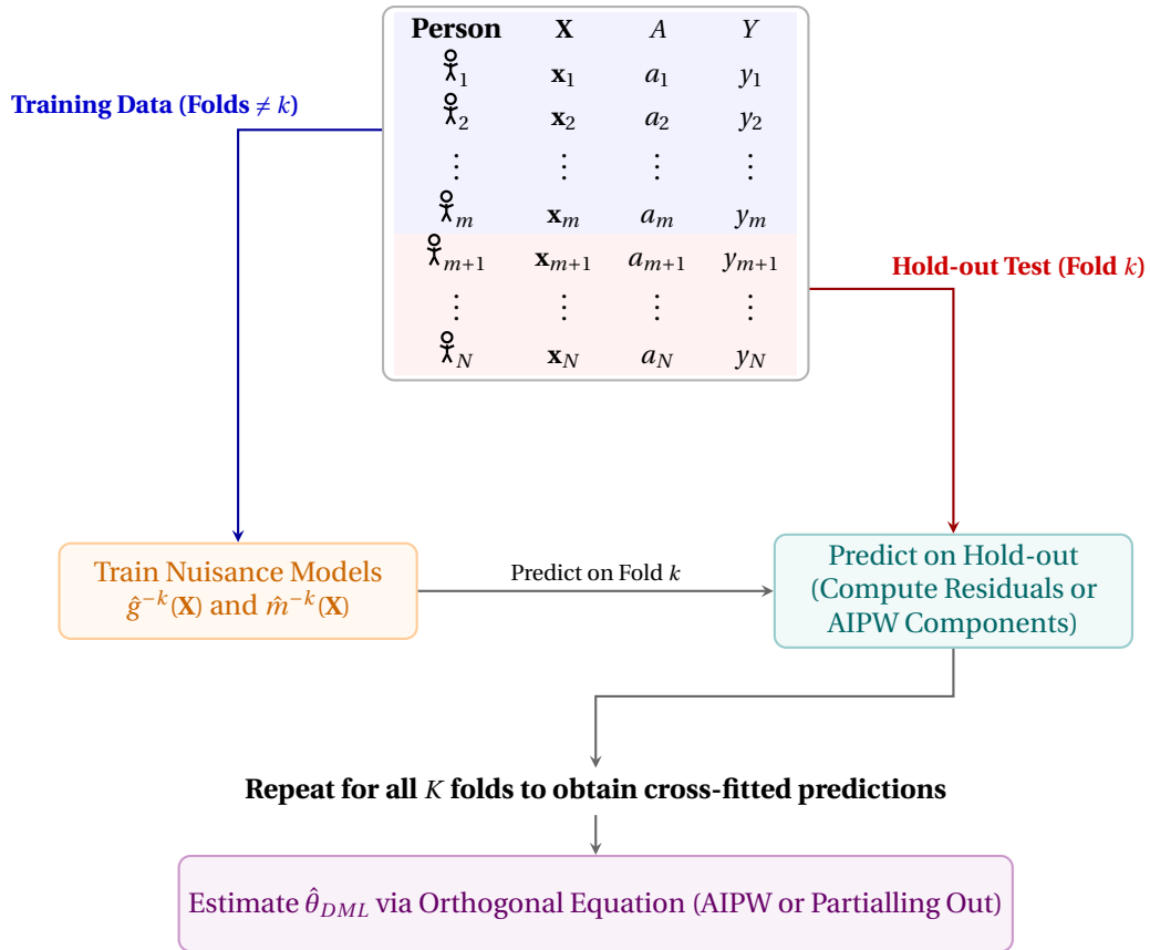
Figure 4.5: The cross-fitting procedure in Double Machine Learning. The dataset is partitioned into training and hold-out folds. For each fold k , machine learning nuisance models are trained exclusively on the blue out-of-fold data. These models are then used to predict and compute the orthogonal components for the red hold-out observations, thereby eliminating own-observation bias.
