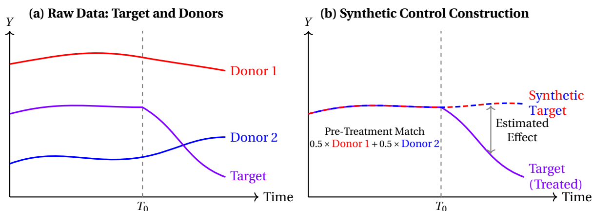
Figure 4.7: Constructing a synthetic control. In (a), the target unit (purple) lies between two donor units (red and blue). In (b), a weighted combination of the donors creates a “Synthetic Target” that matches the pre-treatment trend. The divergence post- T_0 reveals the causal effect.
