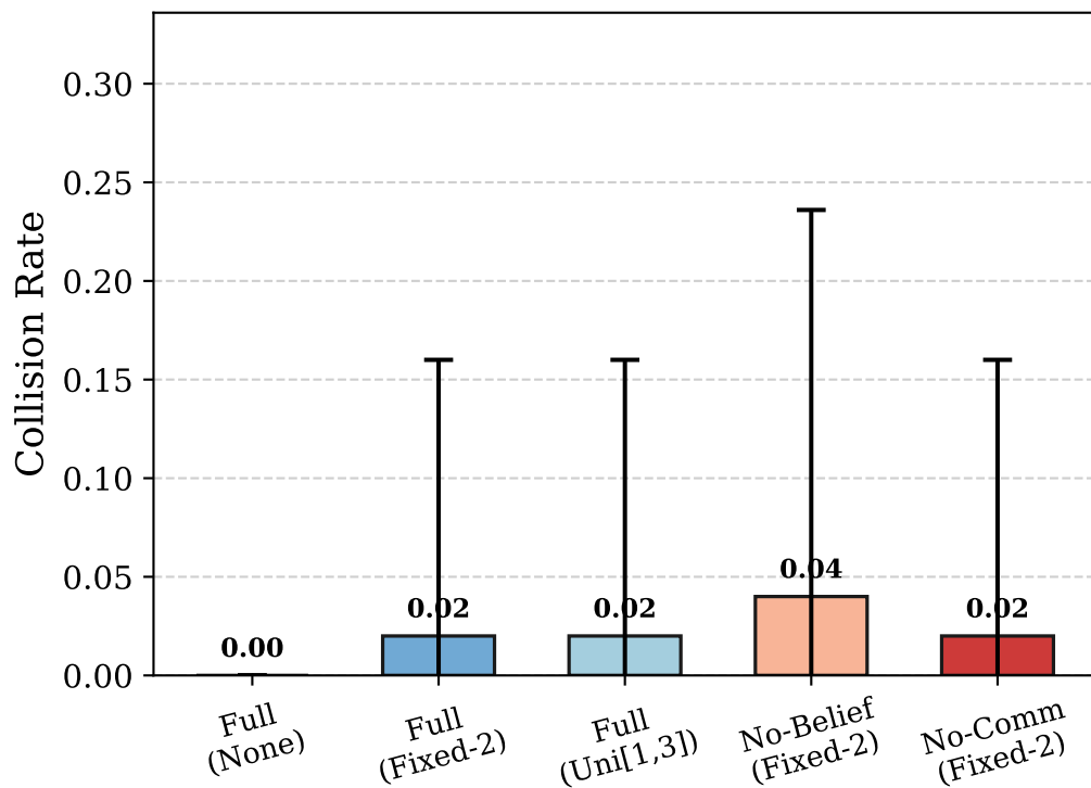
Collision Rate
