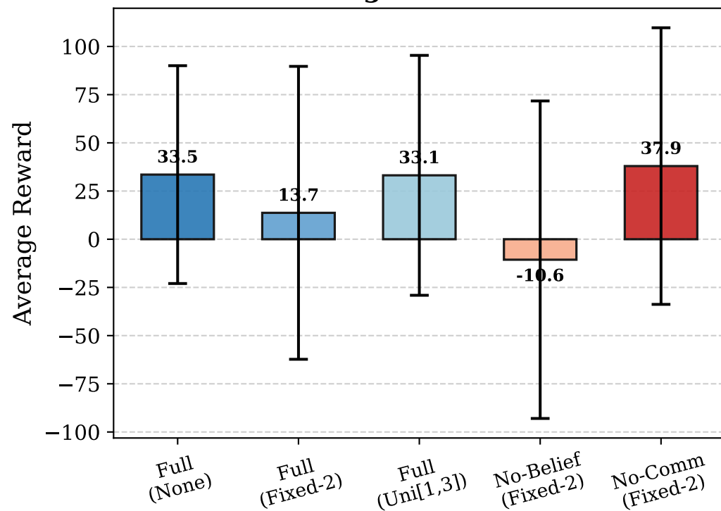
Avg. Reward
