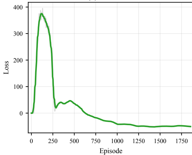
(b) Actor Loss
