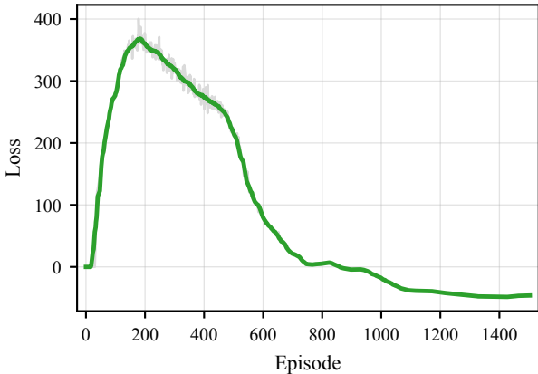
Actor Loss
