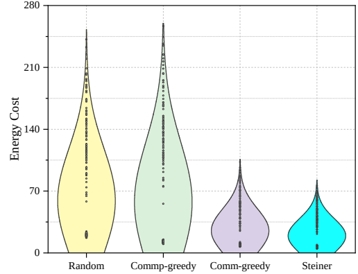
Fig. 10: Energy distribution of Soph Tree.
