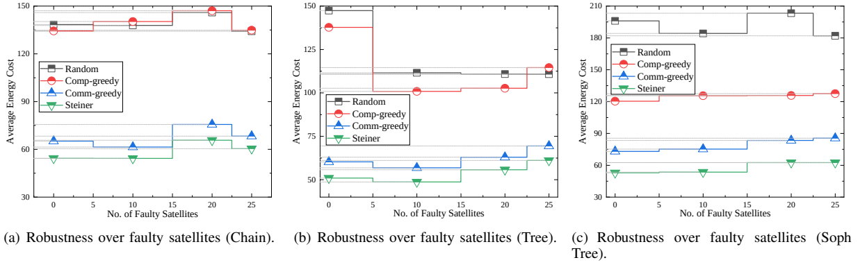
Fig. 4: Performance comparison on energy-cost under different configurations on number of faulty satellites for dynamic service request topologies.
