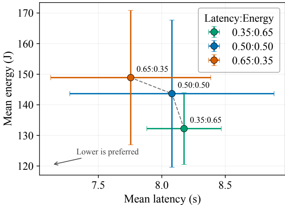
Latency-energy weight sensitivity
