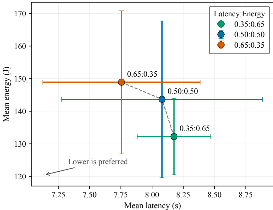
Latency-energy weight sensitivity
