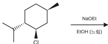
C (menthyl chloride)
