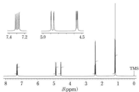
[ ^1H NMR 스펙트럼(400MHz, CDCl_3 )]
