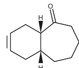
E: cis-bicyclo[5.4.0]undec-9-en-2-one ( \text{C}_{11}\text{H}_{16}\text{O} , 라셀)
