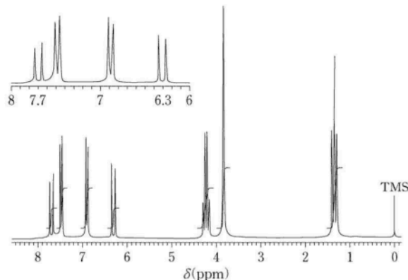
[ ^1H NMR (300 MHz, CDCl_3 )]
