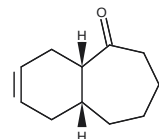
E: cis-bicyclo[5.4.0]undec-9-en-2-one (C 11 H 16 O, 라셀)
