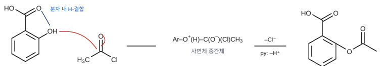
Aspirin (acetylsalicylic acid)
