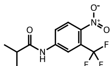
B: flutamide
