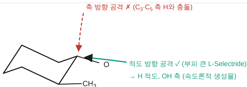
2-methylcyclohexanone
