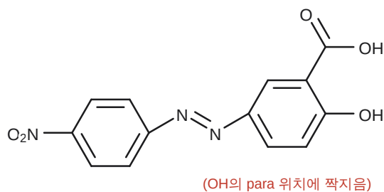
B: 2-hydroxy-5-[(4-nitrophenyl)diazenyl]benzoic acid ( \text{C}_{13}\text{H}_9\text{N}_3\text{O}_5 )
