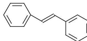
C: (E)-stilbene (trans)
