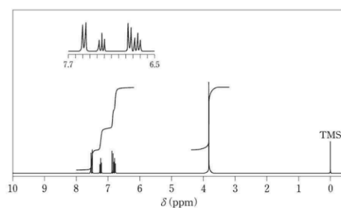
^1\text{H} NMR (300 MHz, \text{CDCl}_3 )
