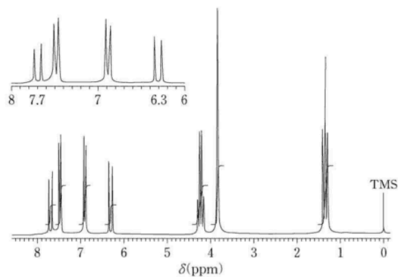
[ ^1H NMR (300 MHz, CDCl_3 )]
