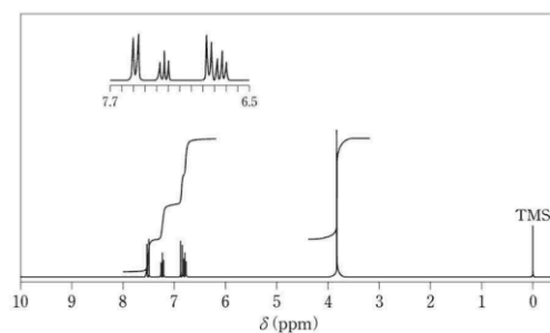
^1\text{H} NMR (300 MHz, \text{CDCl}_3 )
