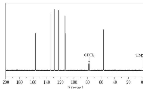
^{13}\text{C} NMR (75 MHz, \text{CDCl}_3 )
