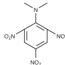
2,4,6-trinitro-N,N-dimethylaniline pK_aH \approx -5
