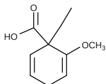
B: 1-ethyl-2-methoxycyclohexa-2,5-diene-1-carboxylic acid
