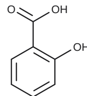
(나) salicylic acid pK_a 2.97
