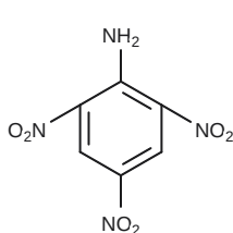
2,4,6-trinitroaniline pK_aH \approx -10 (최소)
