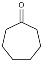
C: cycloheptanone
