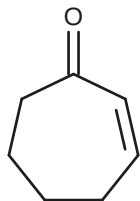
B: cyclohept-2-enone
