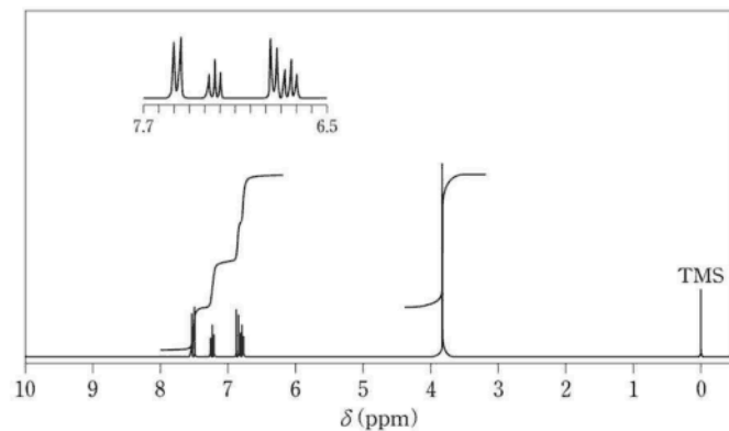
^1\text{H} NMR (300 MHz, \text{CDCl}_3 )
