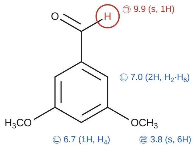
A: 3,5-dimethoxybenzaldehyde (C 9 H 10 O 3 )
