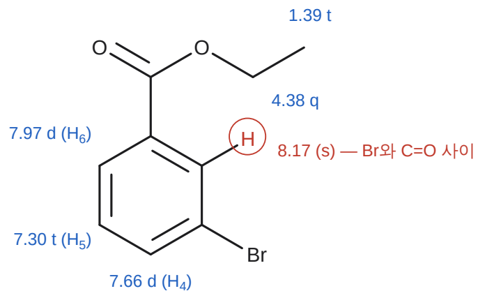
ethyl 3-bromobenzoate (C 9 H 9 BrO 2 )
