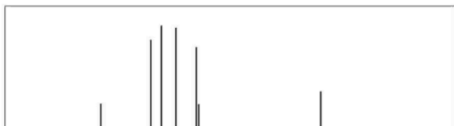
^{13}\text{C} NMR (75 MHz, \text{CDCl}_3 )
