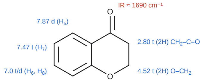
A: chroman-4-one ( \text{C}_9\text{H}_8\text{O}_2 )
