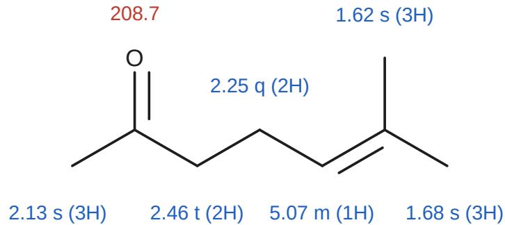
6-methyl-5-hepten-2-one ( C_8H_{14}O )
