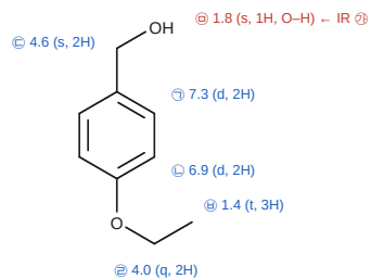
A: 4-ethoxybenzyl alcohol ( C_9H_{12}O_2 )
