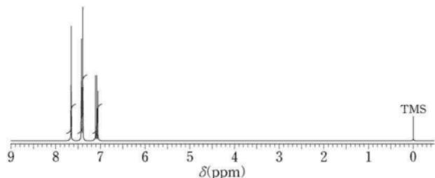
[ ^1\text{H} NMR 스펙트럼 (300 MHz, \text{CDCl}_3 )]
