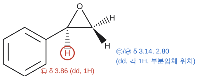
styrene oxide (2-phenyloxirane), C_8H_8O
