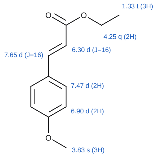
ethyl (E)-3-(4-methoxyphenyl)propenoate (C 12 H 14 O 3 )
