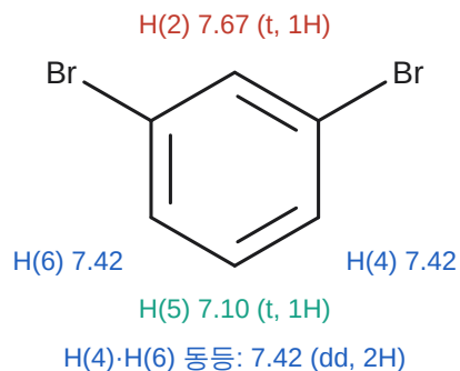
1,3-dibromobenzene (m-dibromobenzene), C 6 H 4 Br 2
