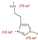
histamine
