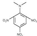
2,4,6-trinitro-N,N-dimethylaniline pKaH ≈ -5
