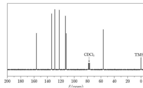
^{13}\text{C} NMR (75 MHz, \text{CDCl}_3 )
