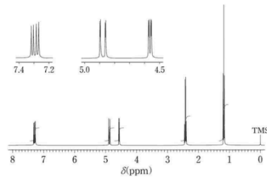
[ ^1H NMR 스펙트럼(400MHz, CDCl_3 )]
