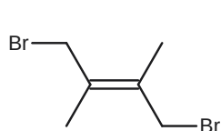
① 1,4-dibromo-2,3-dimethyl-2-butene (E/Z)
