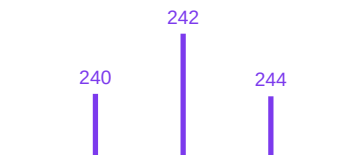
① 1,4-dibromo-2,3-dimethyl-2-butene (E/Z)
