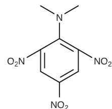
2,4,6-trinitro-N,N-dimethylaniline pK a H ≈ -4.8
