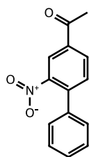
D: 1-(2-nitro-[1,1'-biphenyl]-4-yl)ethan-1-one
