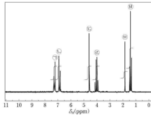
[ ^1H NMR 스펙트럼(90MHz, CDCl_3 )]
