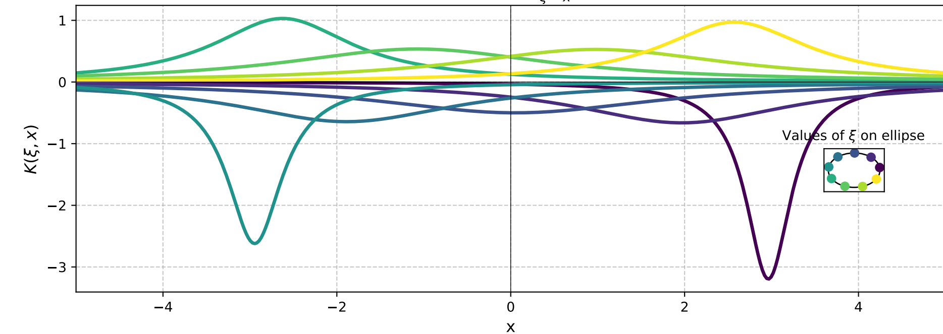
Graph of imaginary part of K(\xi, x) = \frac{1}{\xi-x} with \xi taken on an ellipse
