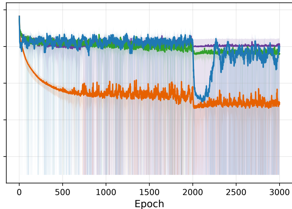
Validation loss (MSE)
