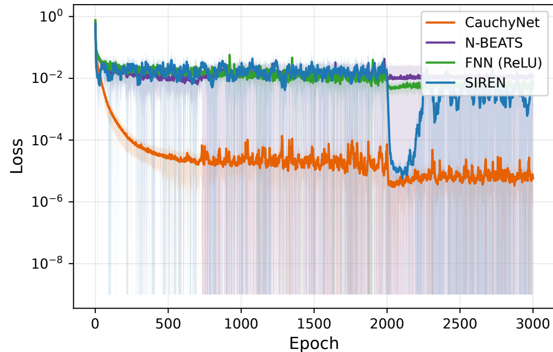
Training loss (MSE)
