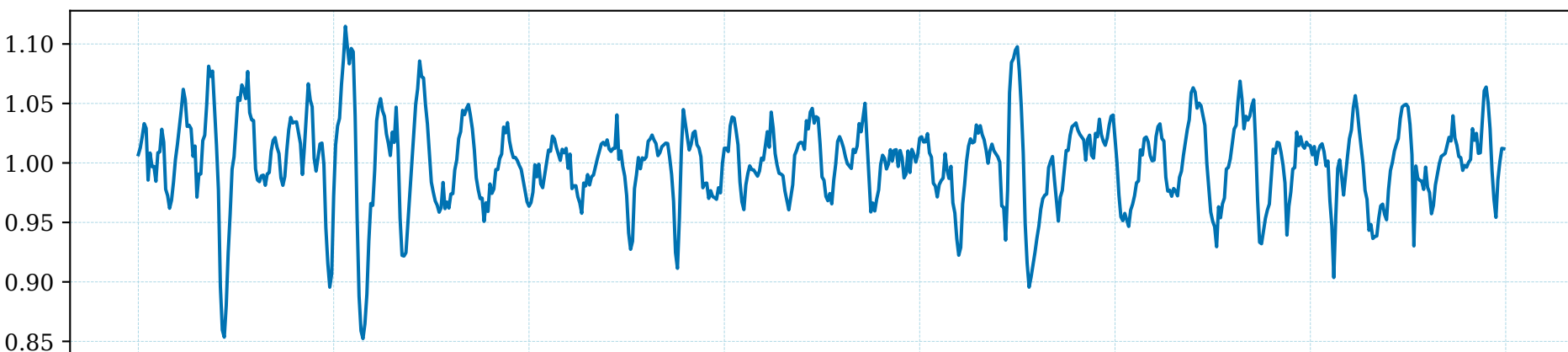
Residual
