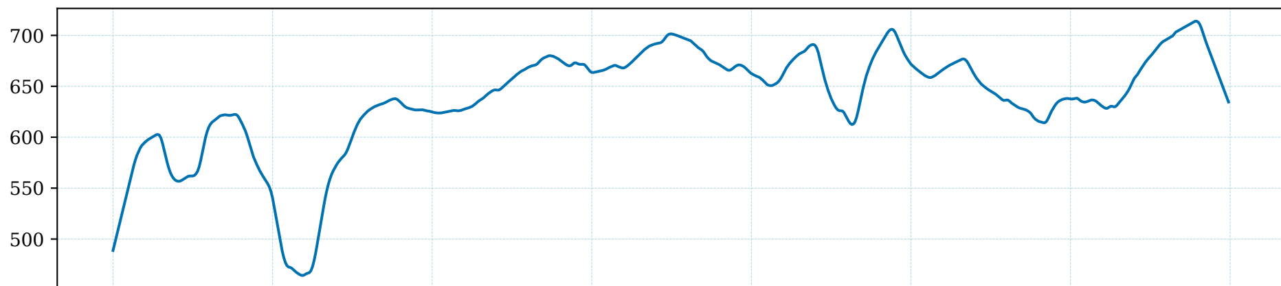
Seasonal
