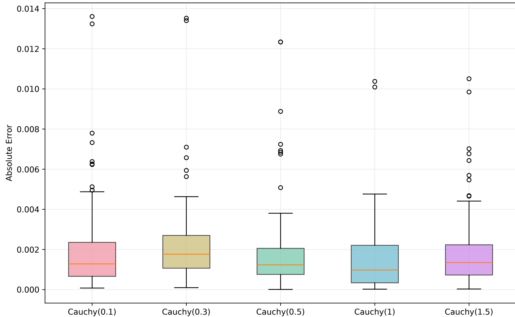
Distribution of Absolute Errors (Test Set)
