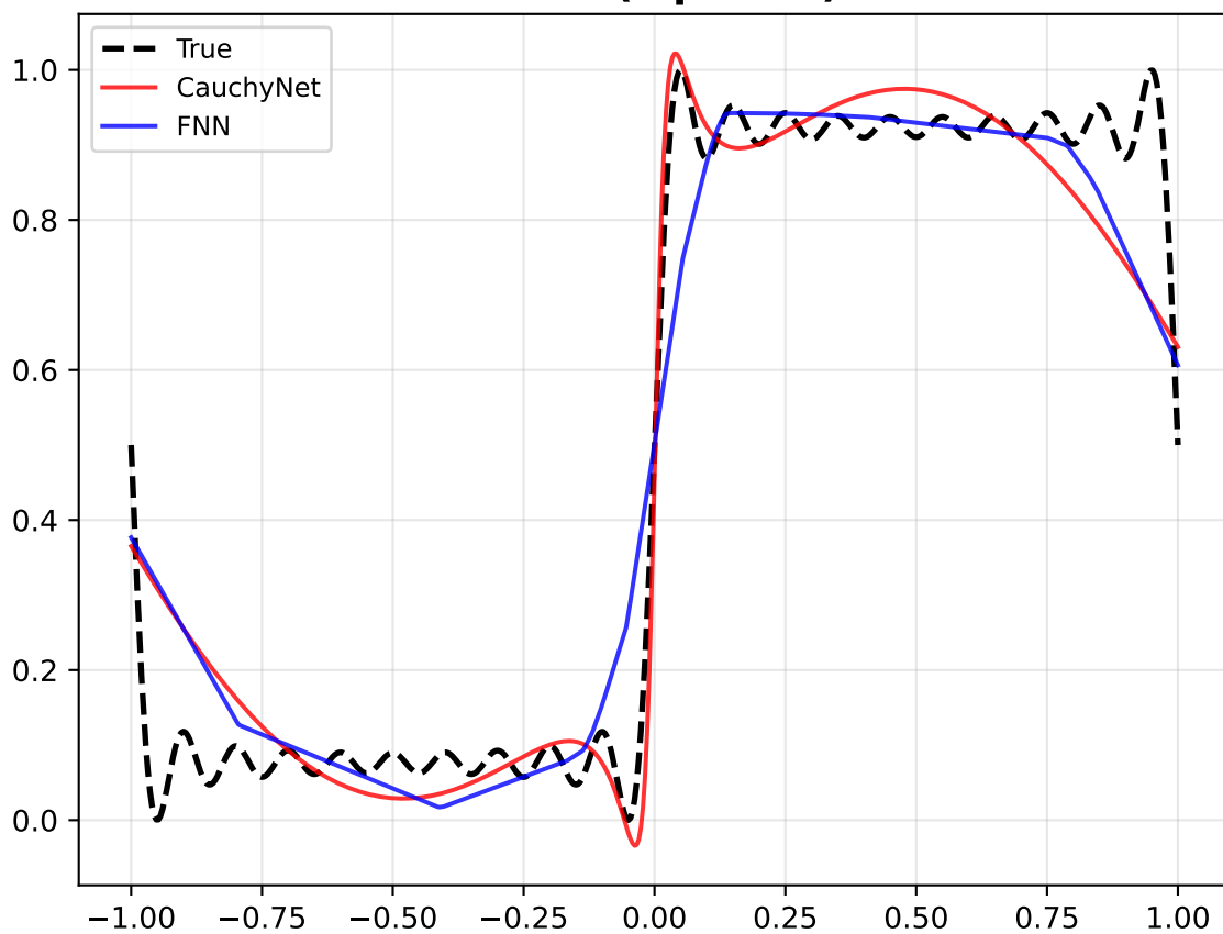
Gibbs (sq wave)
