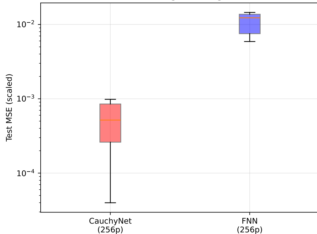
Near-singular target
