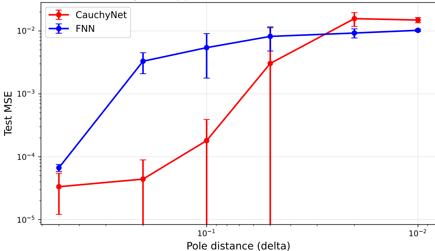
Near-Singular Approximation: MSE vs Pole Distance
