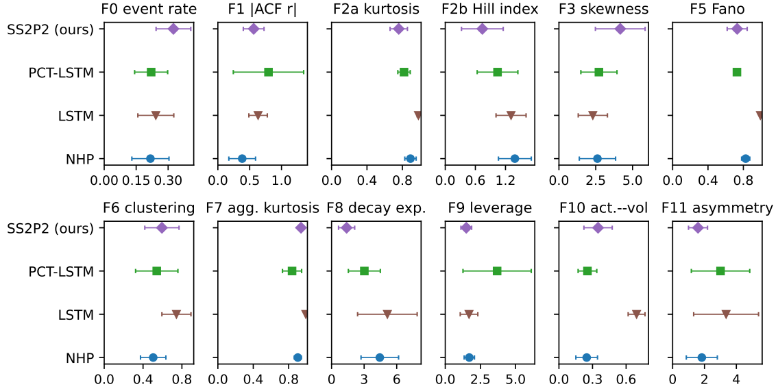
Figure 3: The full stylized-fact battery, pooled across the three assets: relative error vs. real for event rate (F0), Fano factor averaged over 1–50 s scales (F5), and the ten distributional facts F1–F11 (whiskers = 95% CI over asset-checkpoint pairs; roll-out seeds averaged within checkpoint). S2P2 and SAHP omitted: too few calibrated checkpoints.
