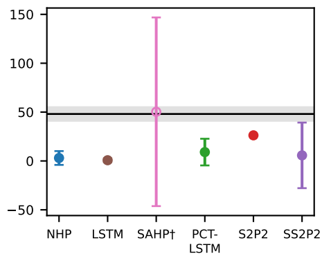
F2a excess kurtosis (heavy tails, > 0 )
