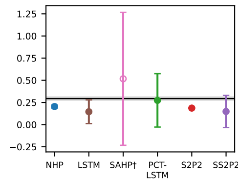
F11 timescale asymmetry (coarse→fine, > 0 )
