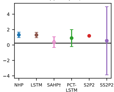
F8 ACF |r| decay exponent
