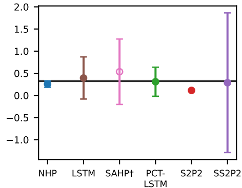
F7 aggregated kurtosis (rescaled, 10s)
