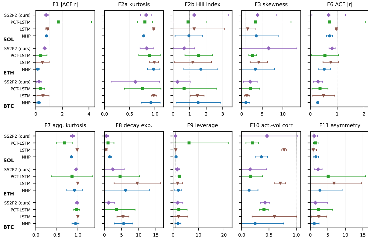
Figure 6: All ten stylized facts across assets: relative error vs. real (dotted line = 100% error; whiskers = 95% CI over checkpoints; roll-out seeds averaged within checkpoint). S2P2 and SAHP omitted where no calibrated checkpoints exist.
