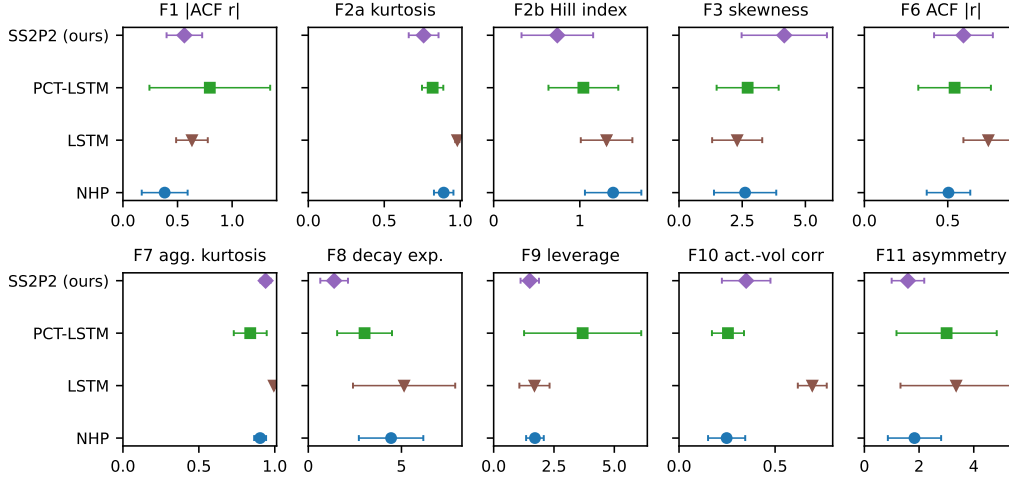
Figure 4: All ten stylized facts, pooled across the three assets: relative error vs. real (whiskers = 95% CI over asset-checkpoint pairs; roll-out seeds averaged within checkpoint). S2P2 and SAHP omitted: too few calibrated checkpoints.
