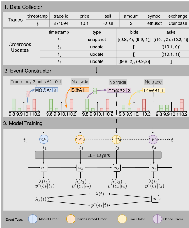
Figure 2: Pipeline. (1) Data collector : synchronized trade records and Level-2 order book updates. (2) Event constructor : consecutive book snapshots are differenced and aligned with trades to emit atomic typed events (Section ). (3) Model training : the event-set sequence drives the state-space backbone (LLH layers) whose continuous-time hidden representation h_t decodes the bounded total rate \lambda(t) and the rate-neutral mark distribution p(e | t) , giving per-type intensities \lambda_e(t) = \lambda(t) p(e | t) .
