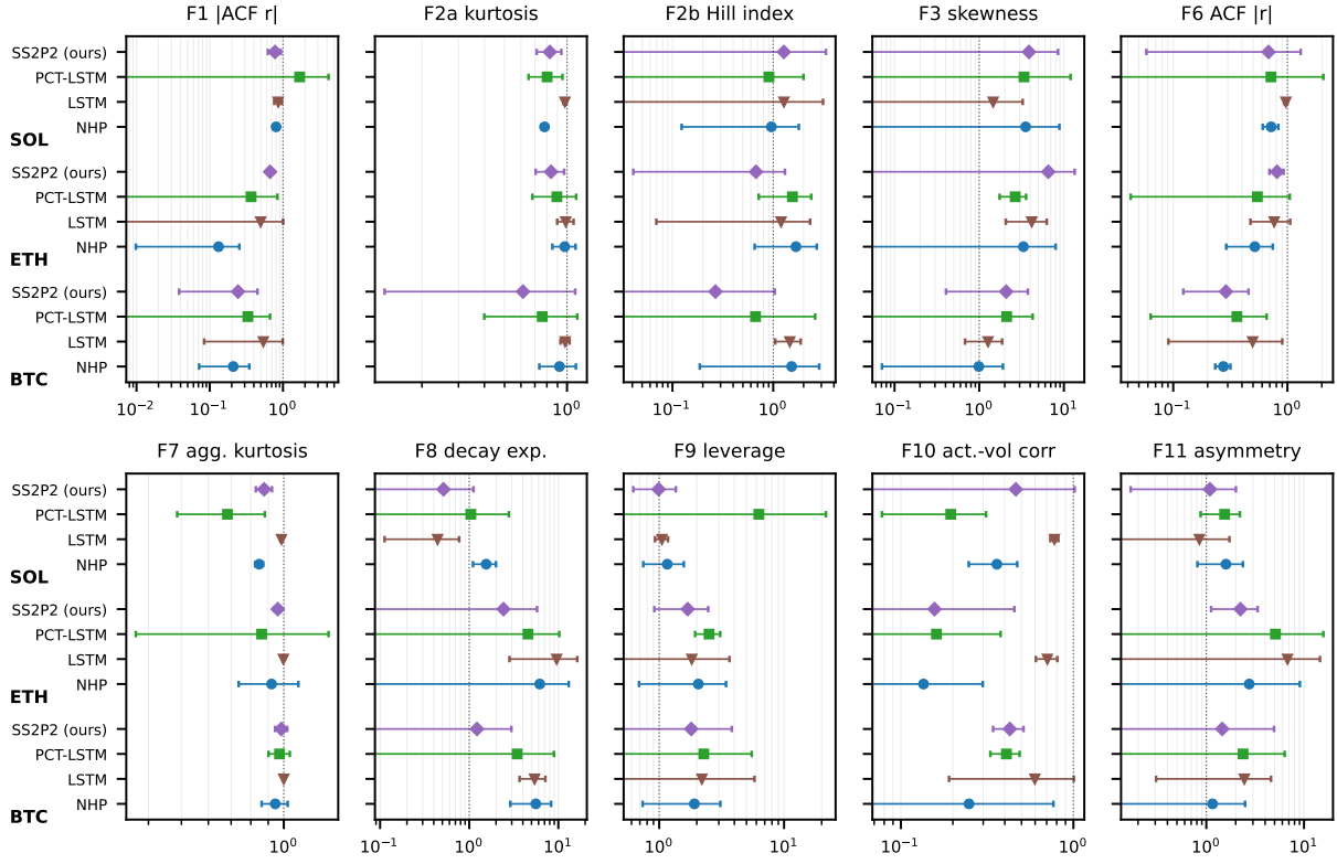
Figure 6: All ten stylized facts across assets: relative error vs. real (log scale; dotted line = 100% error; whiskers = 95% CI over checkpoints; roll-out seeds averaged within checkpoint). S2P2 and SAHP omitted where no calibrated checkpoints exist.
